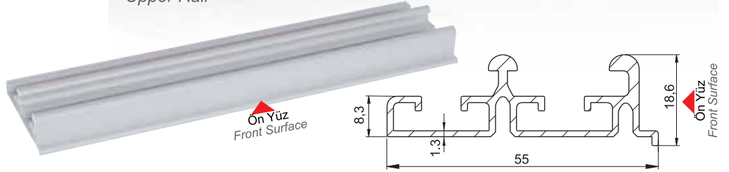
H605 Üst Ray Upper Rail
